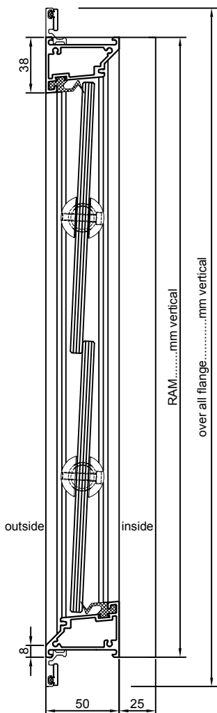
vertical section
