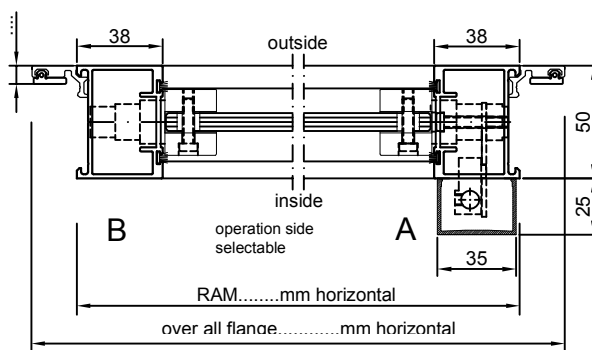
horizontal section
