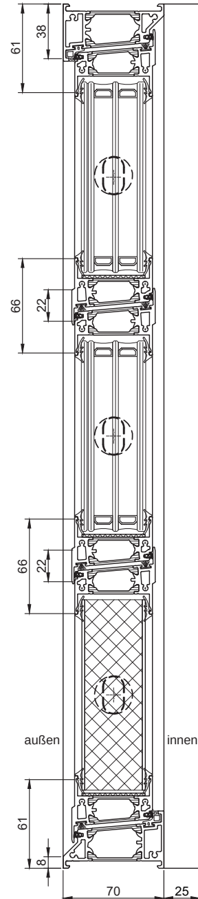
vertical section (shown without control element)
